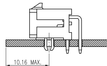
LOCATION DETAIL
