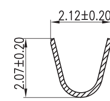
SECTION Z-Z
