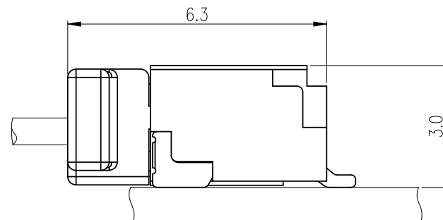
ASSEMBLY LAYOUT SIDE ENTRY TYPE
