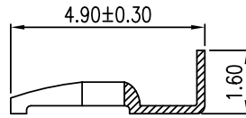
SEC B-B
