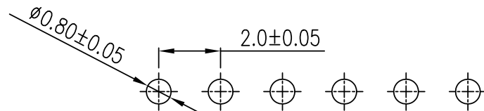
RECOMMENDED PCB LAYOUT (PCB THK=1.0 OR 1.6)
