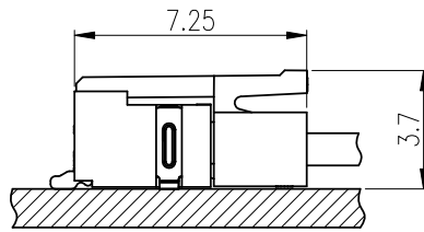
ASSEMBLY LAYOUT SIDE ENTRY TYPE SCALE:1/2
