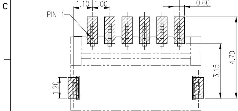
RECOMMENDED P.C.B BOARD LAYOUT GENERAL TOLERANCE ±0.05
