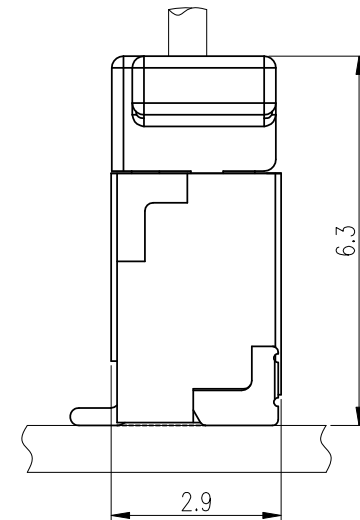
ASSEMBLY LAYOUT TOP ENTRY TYPE
