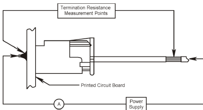
Figure 3 LLCR Measurement Points
