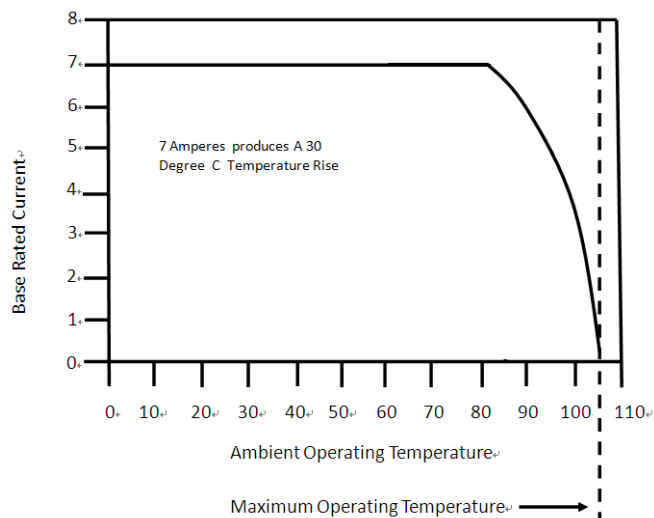
Figure 4 (Current Rating)
