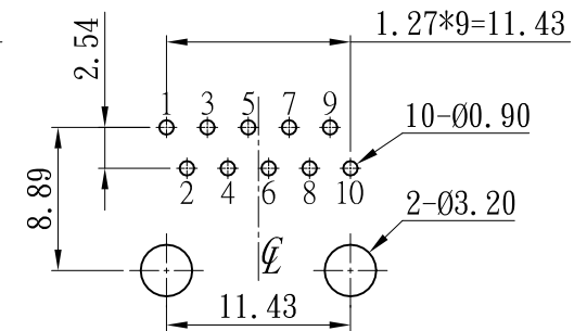
10P10C RECOMMENDED PCB LAYOUT TOLERANCE ±0.05mm(T=1.6mm) TOP VIEW (COMPONENT SIDE)
