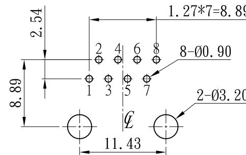
10P8C RECOMMENDED PCB LAYOUT TOLERANCE ±0.05mm(T=1.6mm) TOP VIEW (COMPONENT SIDE)
