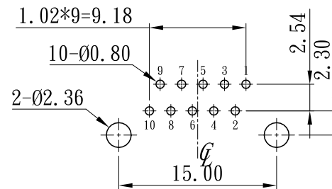
RECOMMENDED PCB LAYOUT(TOP VIEW) (ALL TOLERANCES ARE ±0.05) TOP VIEW (COMPONENT SIDE) 10P10C
