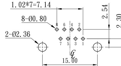
RECOMMENDED PCB LAYOUT(TOP VIEW) (ALL TOLERANCES ARE ±0.05) TOP VIEW (COMPONENT SIDE) 10P8C
