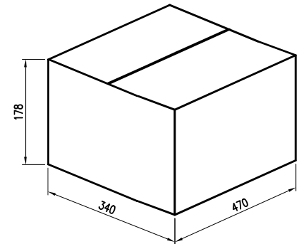
Outer box
