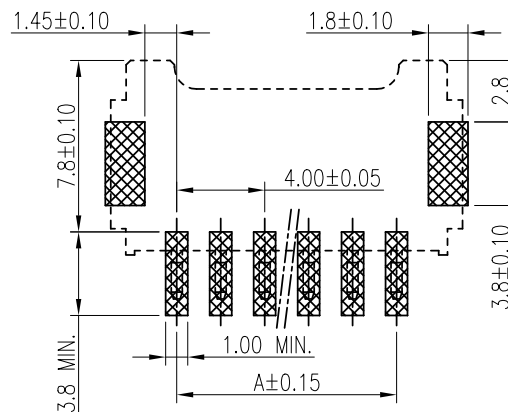
PCB LAYOUT PCB THICKNESS 1.6mm
