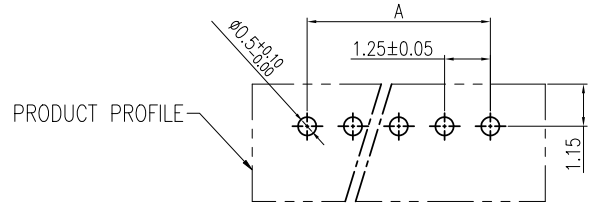
P.C. BOARD LAYOUT (PCB THICK=0.8) TOLERANCES ARE NON-CUMULATIVE:±0.05
