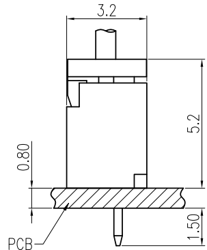
ASSEMBLY LAYOUT TOP ENTRY TYPE
